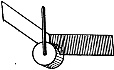
FIG. 62.—Stable. Lateral V and raised axis.
